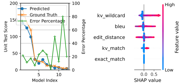
(a) Predicted score of all models, sorted by ground-truth unit test values. (b) SHAP values of different features.
